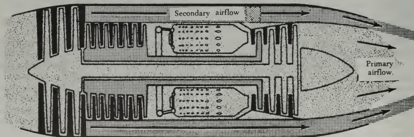
FIGURE 1-69. Forward turbofan engine.
